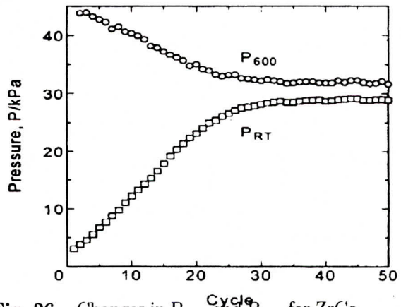
Fig. 26. Changes in P_{600} and P_{RT} for ZrCo-H with heat cycles
