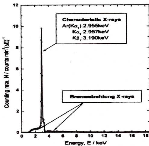
Fig. 21. Typical X-ray spectrum observed for tritium-implanted graphite samples
