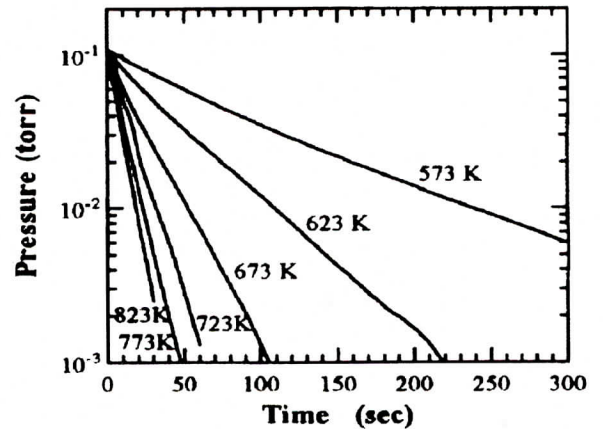
Fig. 8. Methane decomposition-absorption curve by Zr_4Ni
