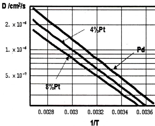
Fig. 32. Temperature dependence of hydrogen diffusion constant for Pd, Pd-4%Pt and Pd-8%Pt
