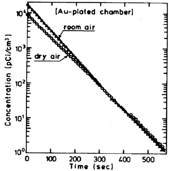
Fig. 3. Reduction of tritium concentration in an ionization chamber made of Au-coated Cu after tritium charge
