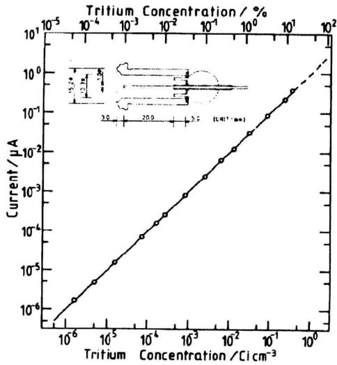
Fig. 17. Cross-sectional view of a small ionization chamber and its calibration curve against tritium concentration
